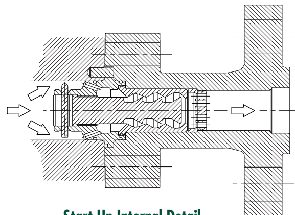
Start Up Internal Detail
