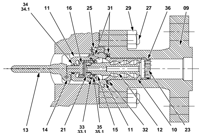
HPM CL600-CL2500 Bypass Detail
