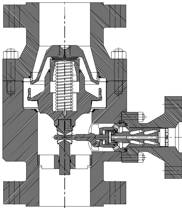
Run Out Protection Detail
