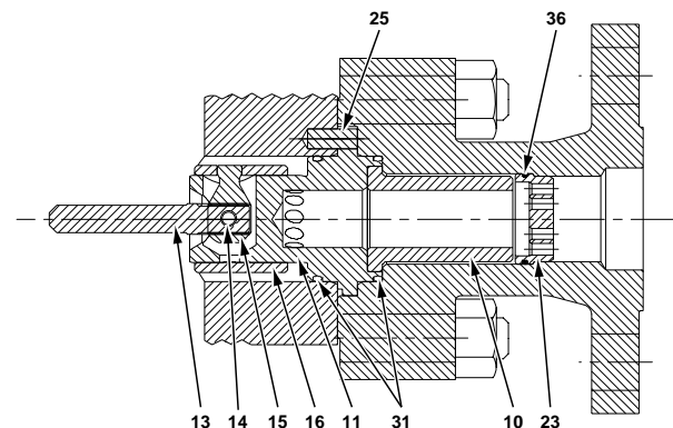
LPM CL150-CL300 Bypass Detail
